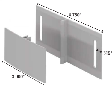
2 pc H-Trim
