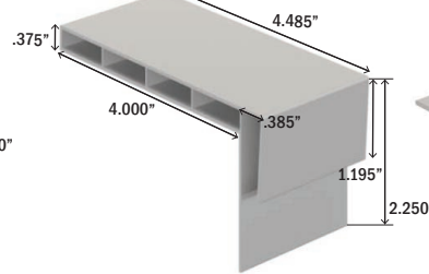
Sill Trim
