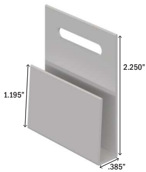
J-Trim
